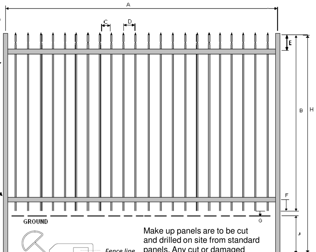
HD post/panel assembly
