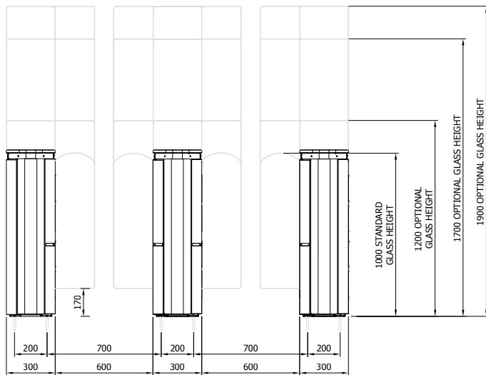
801A Retractable slimlane
